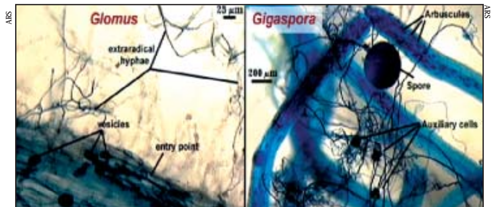
Residue is the food for fungi and bacteria. The fungal hyphae and fine roots surround and stabilize soil aggregates (like glue holding the clay particles together). These aggregates or peds resist breakage when hit by rain or wind.
